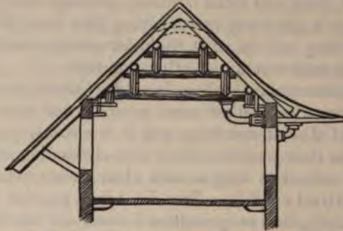
Diagram of Chinese Roof Construction. (From Fergusson.)
